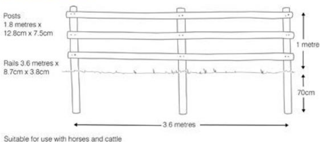
Example of a Post and Rail Fence
