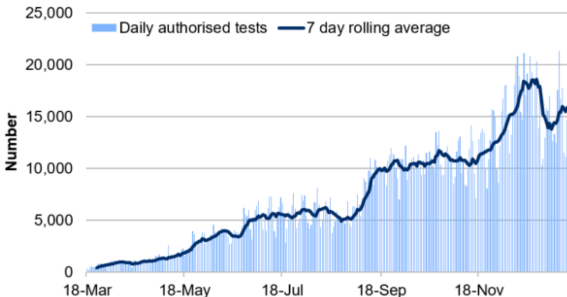
Chart 1: Total number of antigen tests authorised through NHS Wales and non-NHS Wales laboratories as of 17 January 2021
