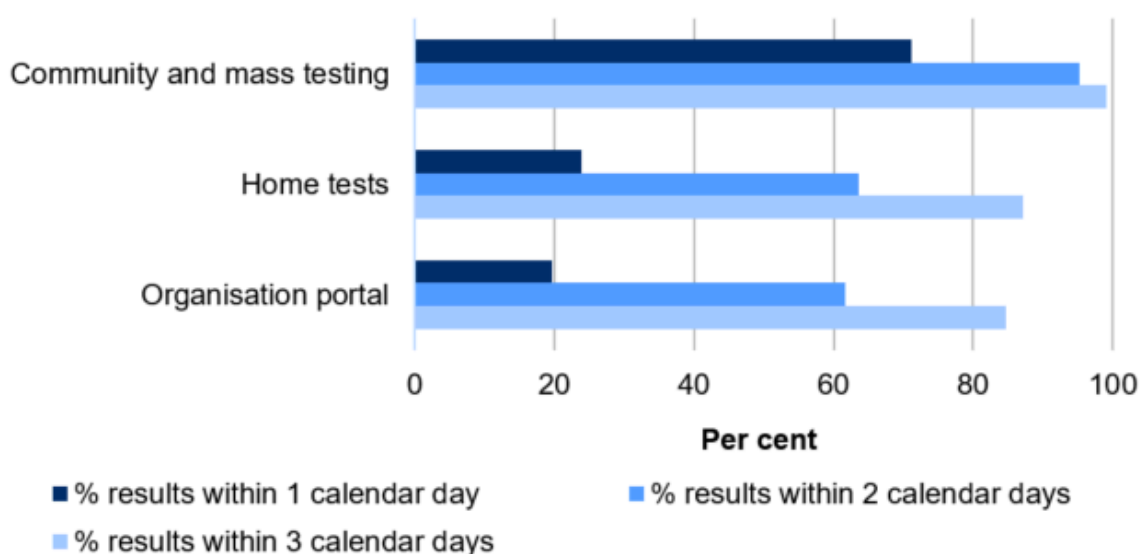
Chart 4: Cumulative proportion of antigen tests authorised from non-NHS Wales laboratories within one, two and three calendar days as at end 17 January 2021
