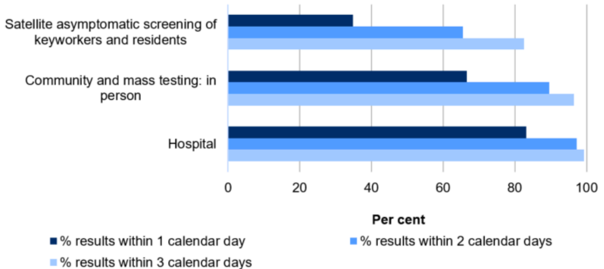
Chart 2: Cumulative proportion of antigen tests authorised from NHS Wales laboratories within one, two and three calendar days as at end 17 January 2021
