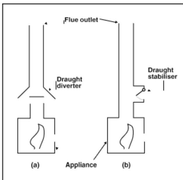
Diagram 3 Draught diverter and draught stabiliser
