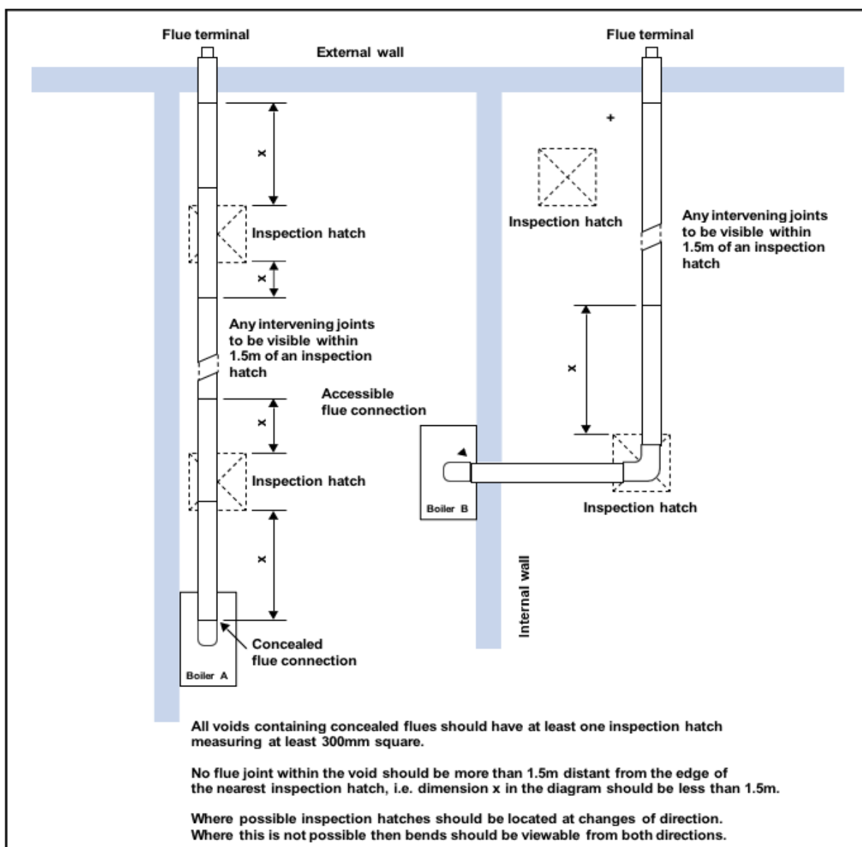
Diagram 14 Example locations of access panels for concealed horizontal flues
